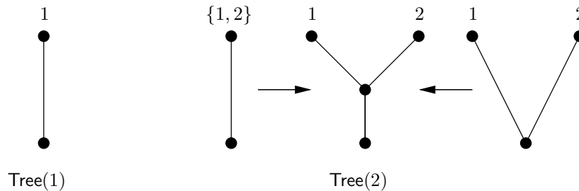
Figure 13: \text{Tree}(1) and \text{Tree}(2) (the arrows represent the direction of the morphisms in \text{Tree}(2) )
