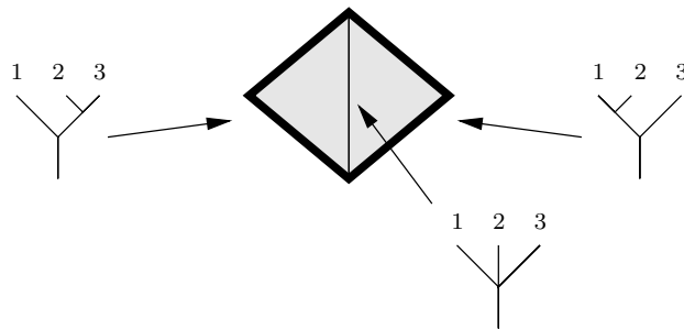
Figure 6: One sixth of B(\mathcal{A}ss_+)(3)
